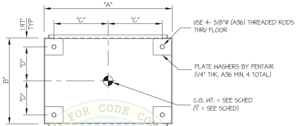
PLANT AT BASE (DUAL ACCESS)
